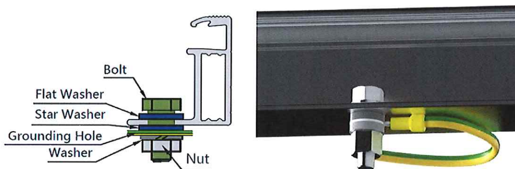
Figure 13. Grounding hole with bolts.
