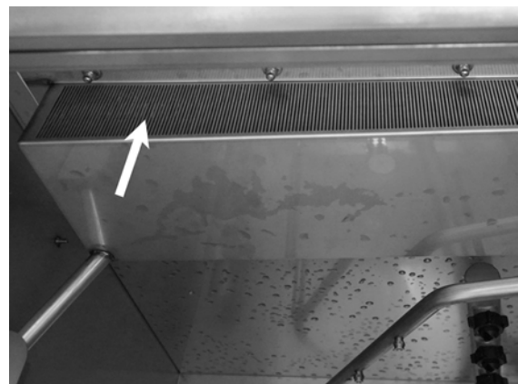
Fig. 44 EcoExchanger as seen inside the machine cabin
