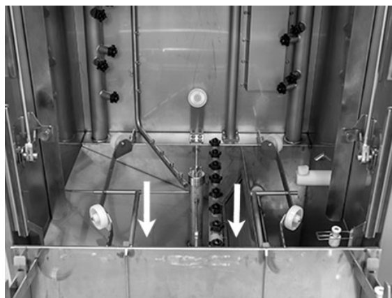
Fig. 41 Clean underneath
