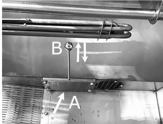
Fig. 39 Sieve for dish washing pump
