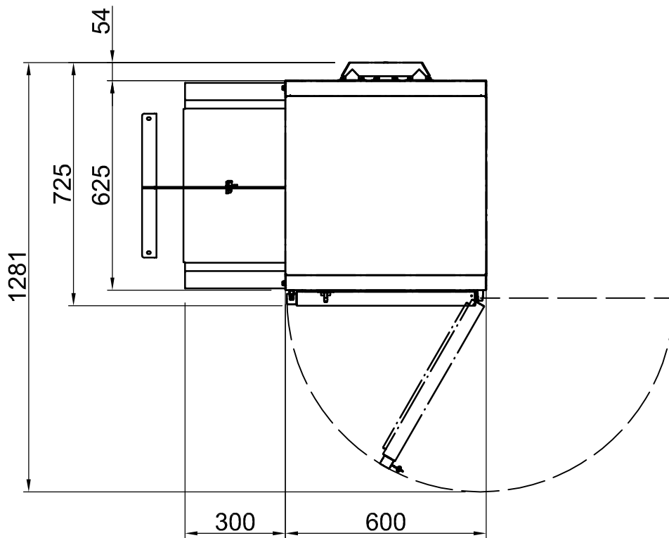
9F51050300RemotePrewashModule, machine driven, Left ST10978-00_R2
